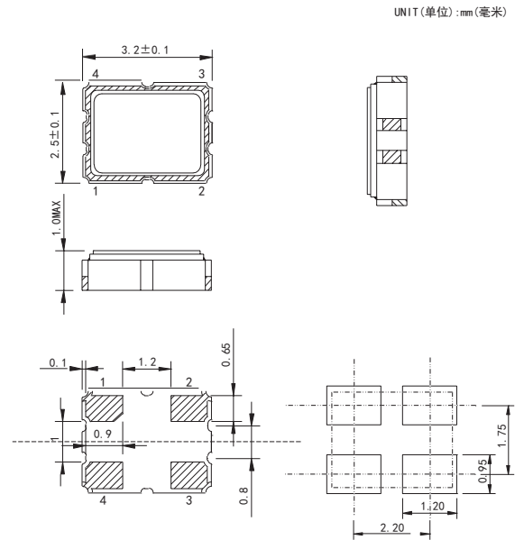
suggested solder pad layout
